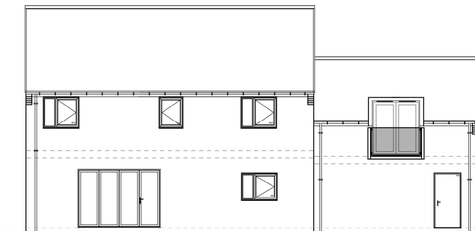
REAR ELEVATION
